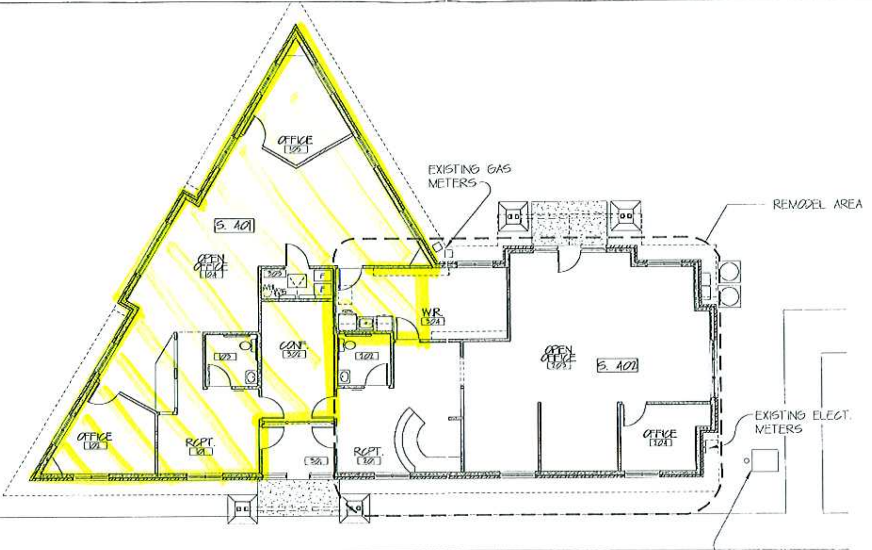
1 EXISTING FLOOR PLAN 1/8" = 1'-0" 0 1'-0" 2'-0" 4'-0" 8'-0"
